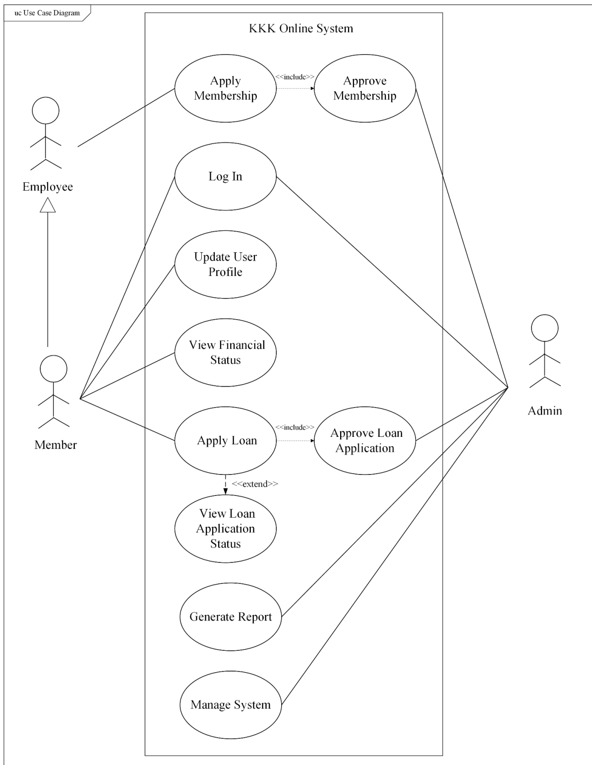
Figure 4: Use Case Diagram for KKK Online System
